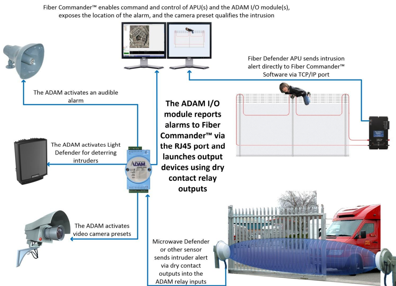
Picture 2: The ADAM Module and Fiber Commander Head End Software, connected to multiple devices
